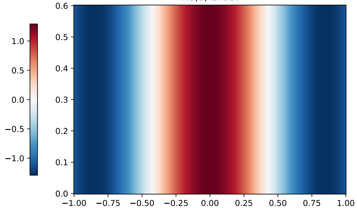
Re(u) Exact
